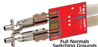
Full Normals
