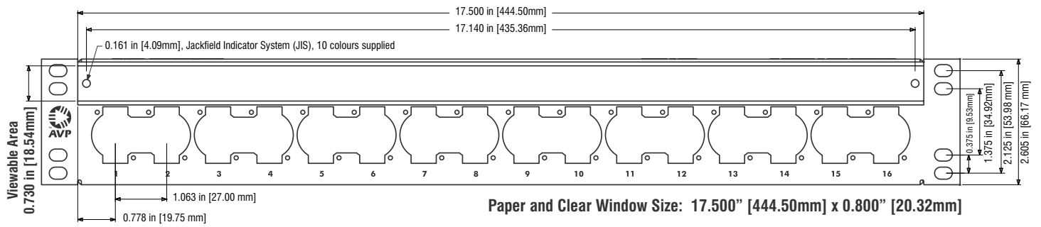
1.5RU, 16 Position, WKME-U116E15-Z Series
